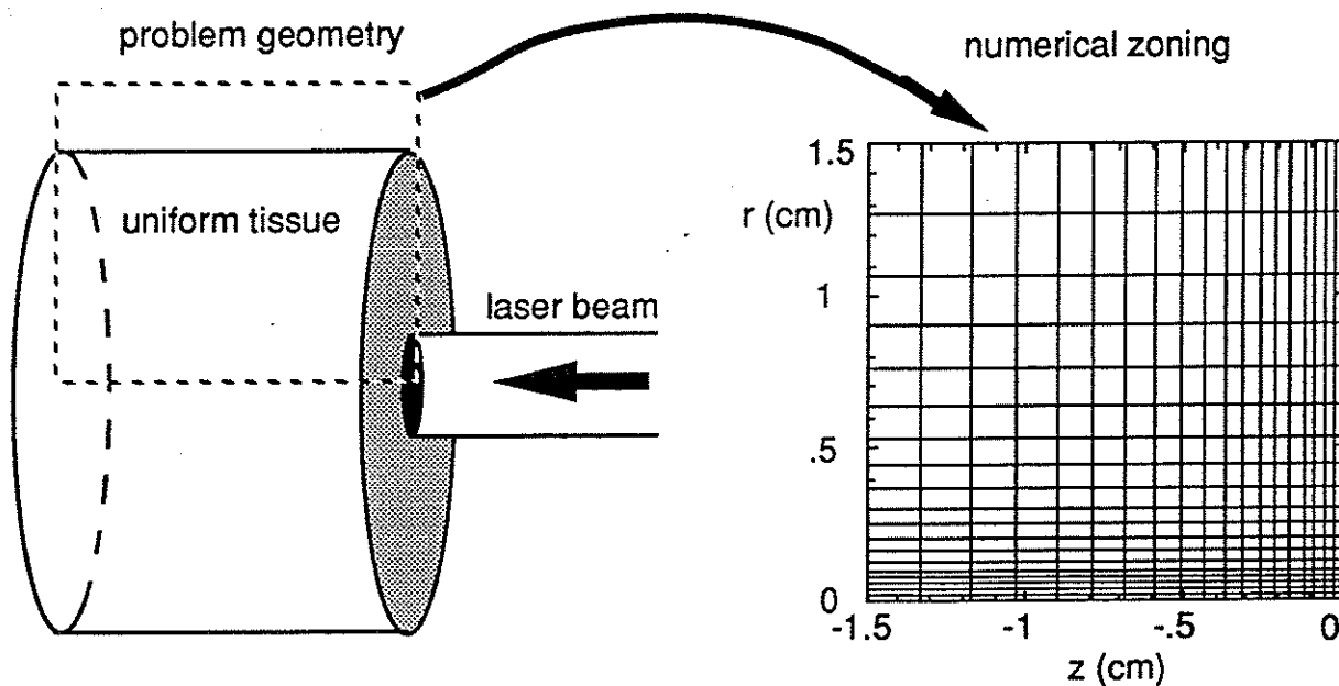
Figure 3. The laser-tissue irradiation is modeled in cylindrical geometry with fine zoning near the laser spot and course zones far from the spot.
