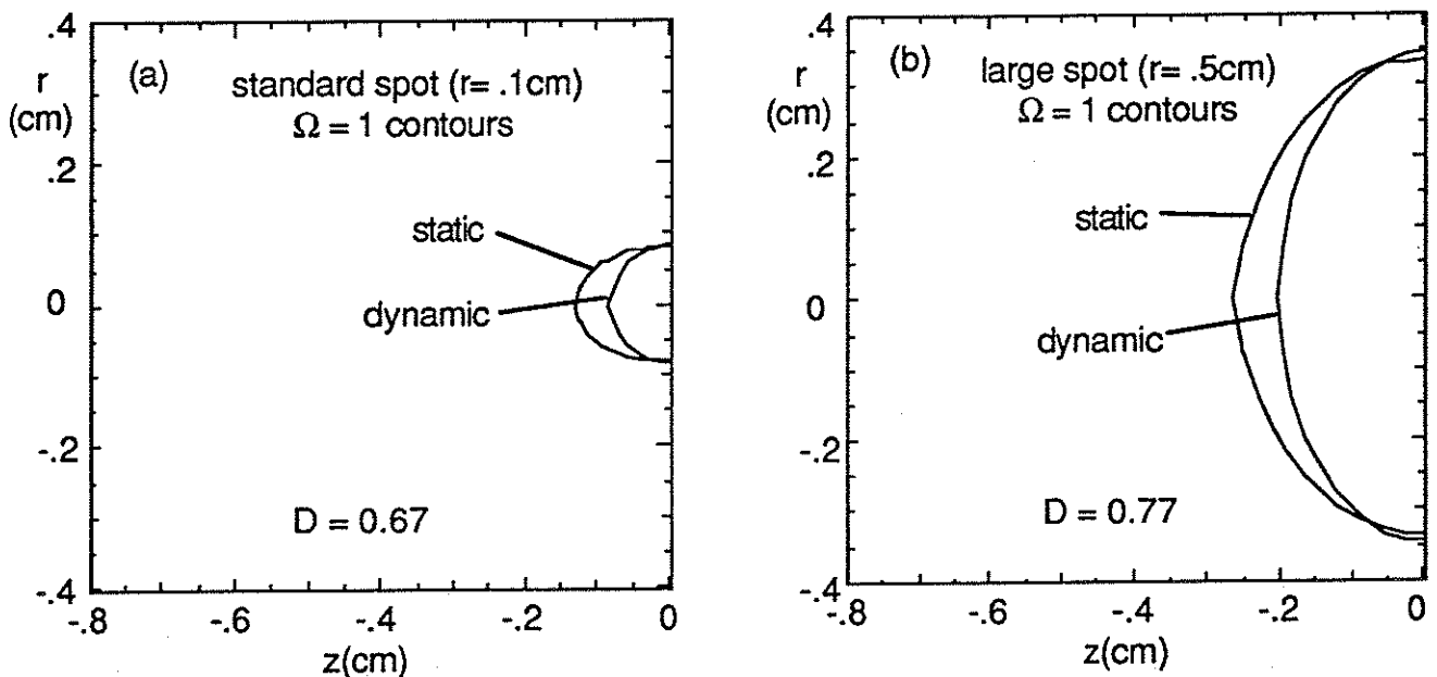
Figure 6. The size of the damage regions is reduced by dynamic optics, as shown for the standard case in Fig. 6a and for a case with a large spot in 6b. The effect of dynamic optics is greater for the standard spot than for the large spot. All curves are for the end of the pulse (at 60 s).
