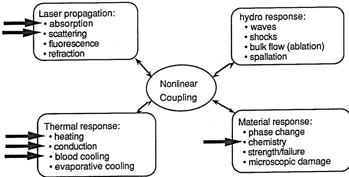
Figure 1. LATIS models laser-tissue interactions considering four areas of coupled physical processes. The arrows indicate features used for the present simulations. Features such as the hydro response are being developed for future use in tissue ablation applications.
