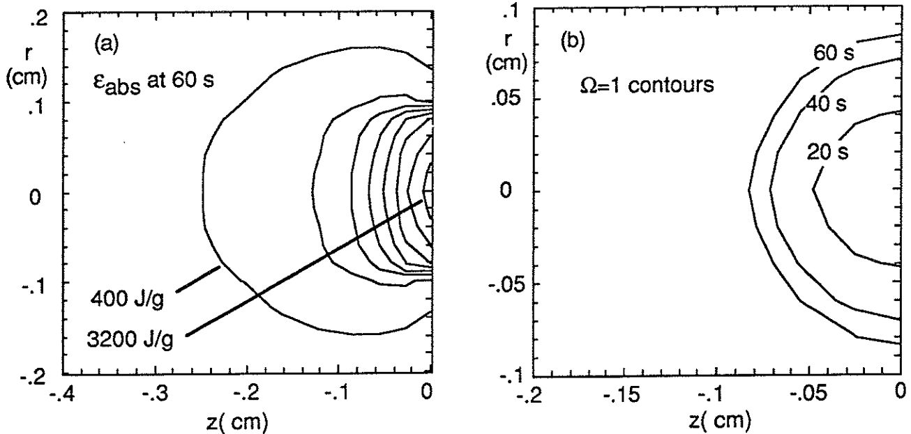
Figure 5. The total absorbed energy density integrated over the 60 s pulse is shown in Figure 5a. Laser and tissue conditions are for the standard case. This pattern reflects the light distribution. The damage region ( \Omega=1 ) is shown at various times during the pulse in 5b. It grows due to heat diffusion and time-accumulation of damage.
