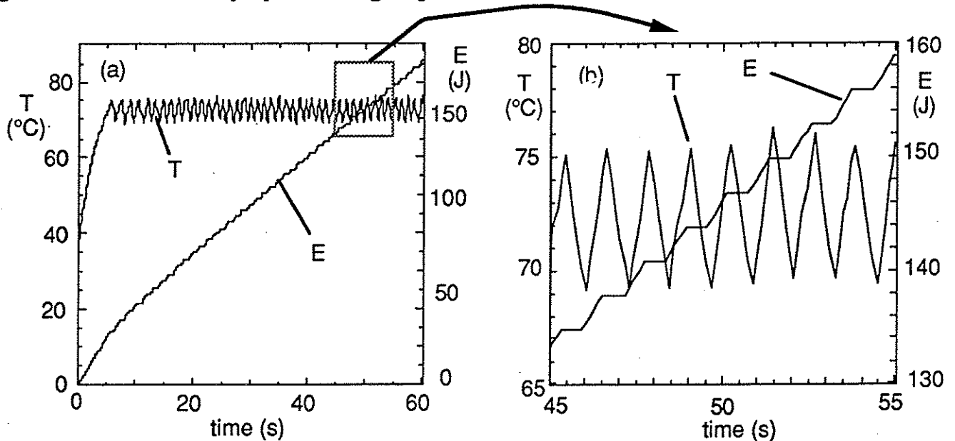
Figure 4. The surface temperature is kept within a desired range by a thermostat function. Here the range is between 70 and 75 °C. The time integrated laser energy shows the periods when the laser is off as flat sections.
