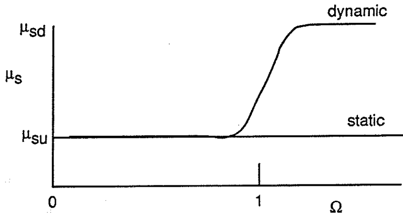
Figure 2. The scattering coefficient varies with damage integral. For static optics cases the scattering coefficient is kept fixed at the undamaged value.
