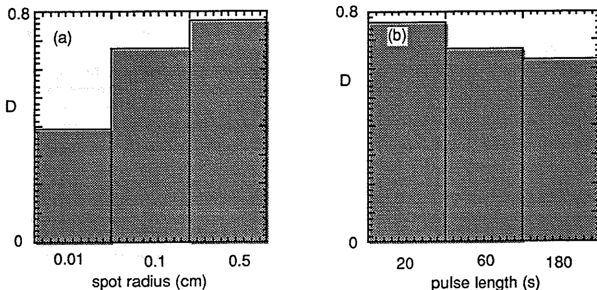
Figure 7. Variation of the damage ratio with spot radius (a) and pulse length (b). The variations can be understood by comparing the spot size to the laser penetration depth and the pulse length to the damage timescale at the surface temperature.
